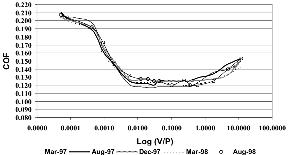
Long-term stability of the Stribeck curves
